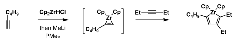
Figure 4. Examples of metallacycle-mediated cross-coupling reactions.
