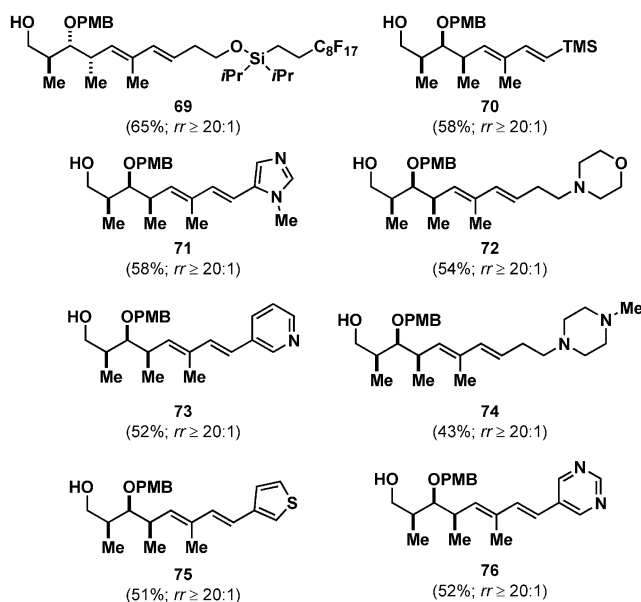
Figure 15. Some functional group compatibility in the Class I alkoxide-directed reductive cross-coupling reaction of internal alkynes with terminal alkynes.
