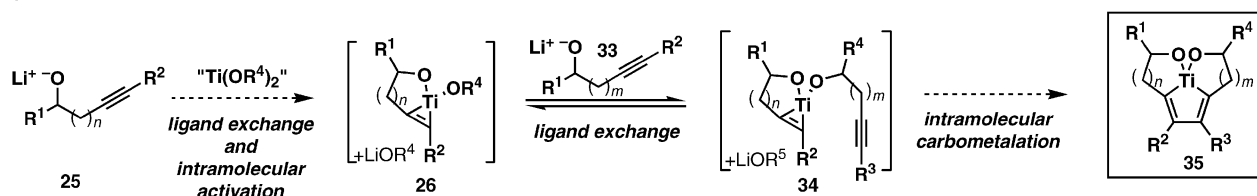
Figure 12. Design of alkoxide-directed reductive cross-coupling reactions.
