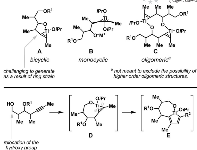
Figure 14. Empirical model for regioselectivity.
