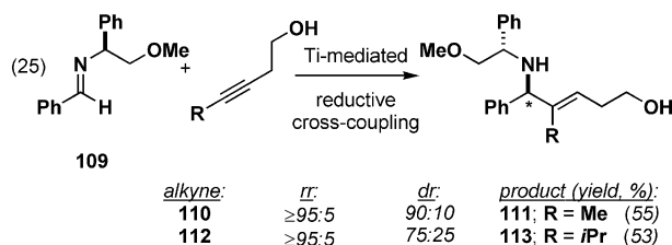
Figure 20. Asymmetric Class II alkoxide-directed reductive cross-coupling reaction.
