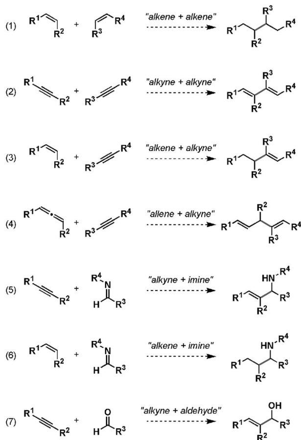
Figure 1. A small subset of possible bimolecular C–C bond forming processes based on reductive cross-coupling.
