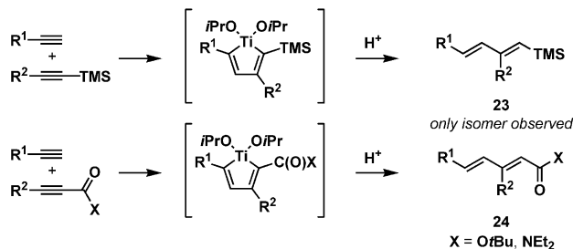
Figure 9. Methods for the control of regioselection in the metallacycle-mediated coupling of disubstituted alkynes with terminal alkynes.
