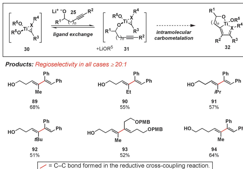
Figure 17. A highly regioselective reductive cross-coupling reaction between internal alkynes.
